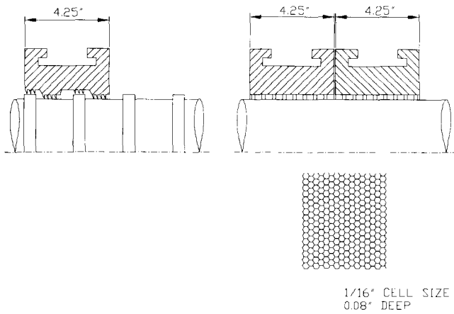
Figure 20. Balance Piston Modification from a Stepped Laby to a Straight Honeycomb.
