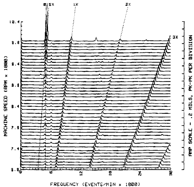
Figure 16. Subsynchronous Vibrations with Dry Gas Seals [11].
