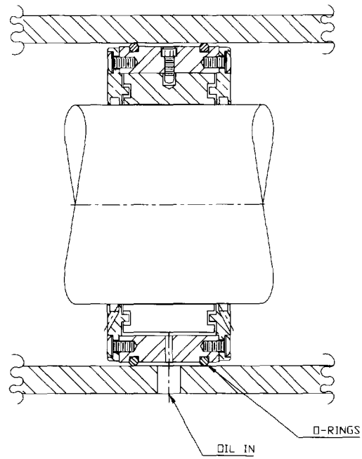
Figure 4. Combination Tilt Pad Bearing and O-Ring Supported Squeeze Film Damper.
