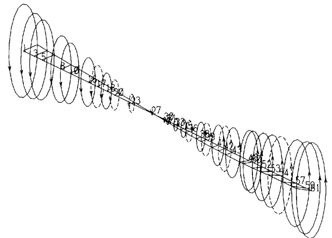
Figure 19. Second Forward Mode with Straight Honeycomb Seal.
