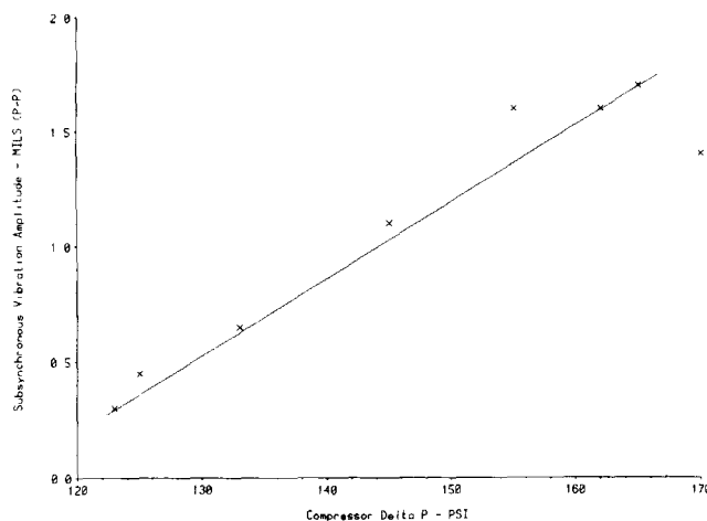
Figure 25. Hydrogen Recycle Compressor Plot of Subsynchronous Vibration Amplitude Vs Pressure Rise.
