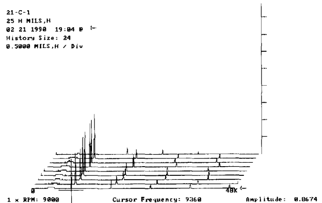
Figure 26. Vibration Spectrum with Honeycomb Seals.
