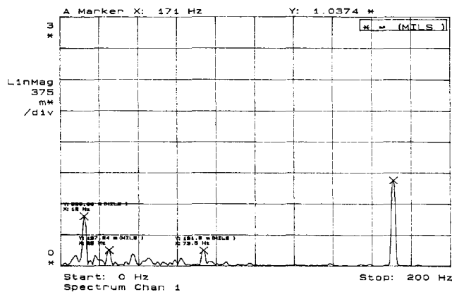
Figure 8. Subynchronous Vibrations with Combination Tilt Pad Bearing and Squeeze Film Damper.
