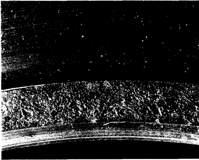
Figure 11. Closeup View of the Floating Oil Seal Ring.
