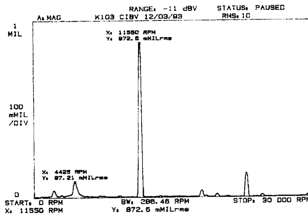
Figure 25. A Vibration Plot at the same Bearing Location on the Subject Compressor with the Pocket Damper Labyrinth Installed and after a Severe ESD Surge Excursion.
