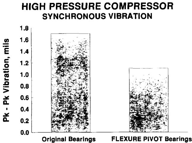
Figure 16. Synchronous Vibration Levels with Two Types of Bearings—HPC.
