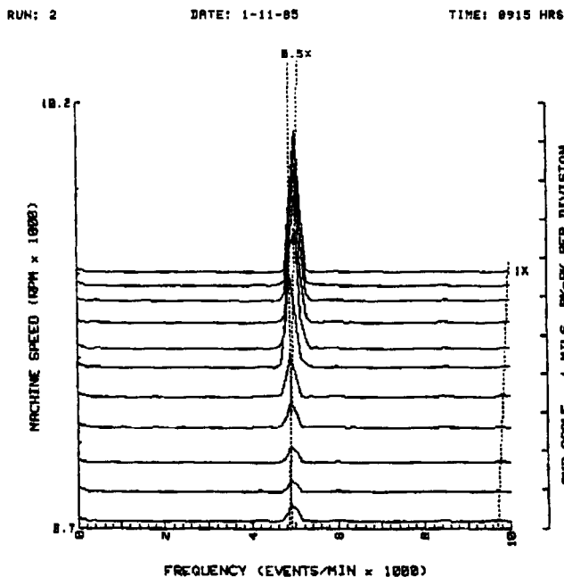
Figure 24. A Waterfall Plot at the Inboard Bearing, Vertical Probe Showing High. Vibration at Subynchronous Frequency after an ESD on another Compressor in the Set.
