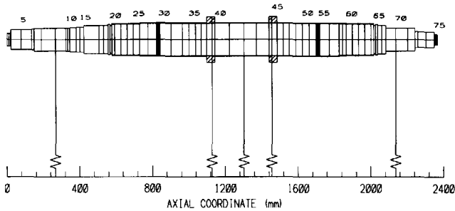
Figure 7. LPC Rotor Model.
