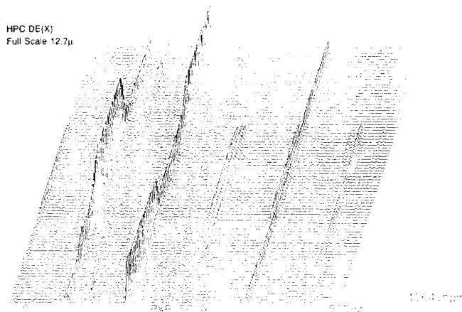
Figure 17. Cascade Plot of HPC Vibration before Modification.
