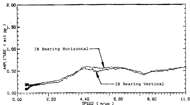
Figure 23. Coastdown Data with the Pocket Damper Center Seal.
