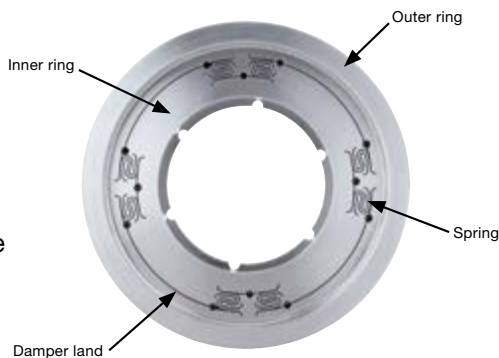
Figure 1: ISFD design
